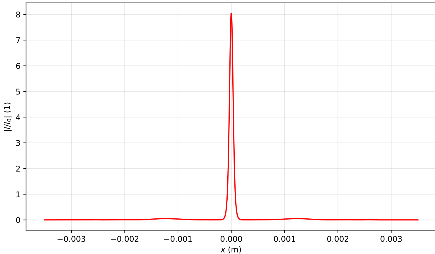
Intensity profile I(x, y = 0, z = 0.955)/I_0 , P_{in}=7.0P_{cr} , artificial time
